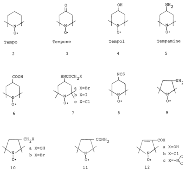
Figure 1. Structures of most frequently used nitroxyls.
